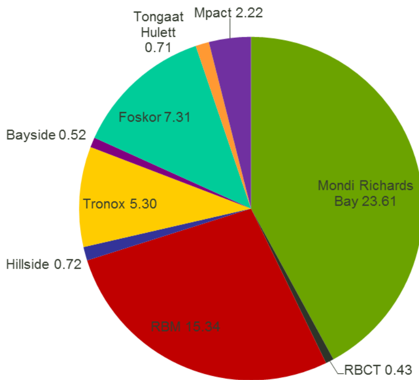
Figure A-3 | Current Industrial Usage (million m³/a)
